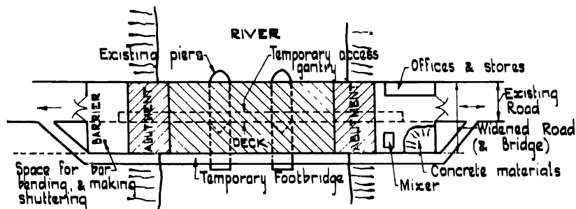
Fig. 269.—Arrangement of Plant for Replacement and Widening of Bridge on Congested Site.
